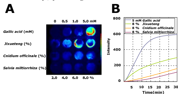
Figure 6: Effects of herbal medicines on photon emission (A) and photon emission intensities (B) in the presence of the oxidant \text{HO}^\cdot . The reaction mixture contained X (250 \mu\text{L} ), Y (100 \mu\text{L} ) and Z (250 \mu\text{L} ) reagents in a 12-well plate (A). The color bar in (A) shows light emitting intensity that is antioxidant activity, and the red in top of color bar shows the highest antioxidant activity. Luminescence was initiated by adding the concentration-fixed XZ mixture into various concentrations of the Y solution. These experiments were performed in the presence of the oxidant \text{HO}^\cdot (X) + a hydrogen donor, an 8% water extract of a herbal medicine ( Jixueteng , Cnidium officinale and Salvia miltiorrhiza ) or 5 mM gallic acid (Y) + mediator (Z) (antioxidant activity increased as the emission intensity increased).
